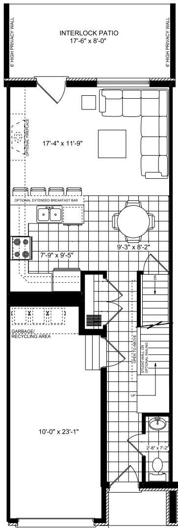
MAIN FLOOR
